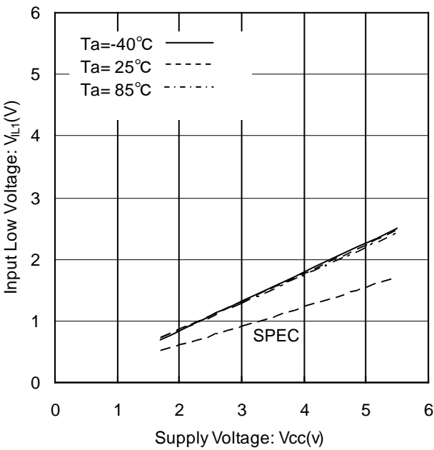
Figure 5. Input Low Voltage1,2 vs Supply Voltage (A1, A2, SCL, SDA, WP)
