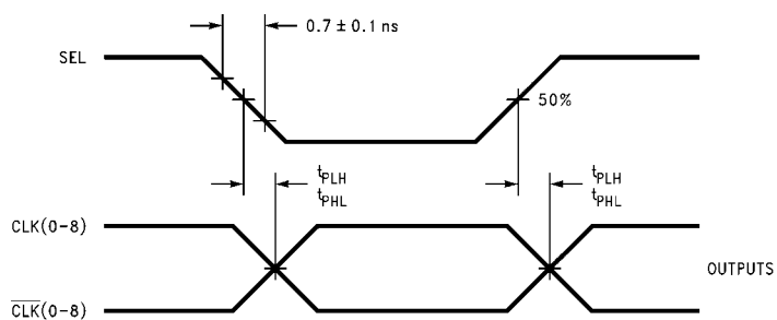
FIGURE 2. Propagation Delay, \overline{\text{EN}} to Outputs
