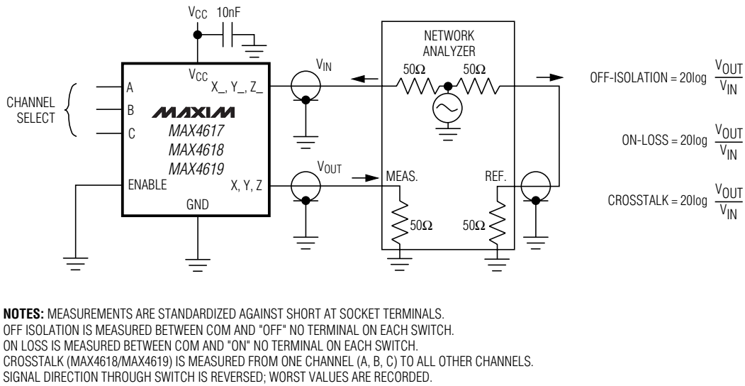
Figure 6. Off-Isolation, On-Loss, and Crosstalk
