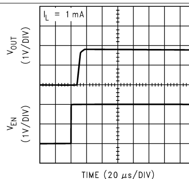
Figure 10. Enable Start-Up Time
