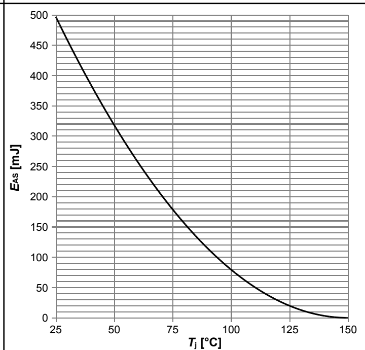
Diagram 16: Avalanche energy
