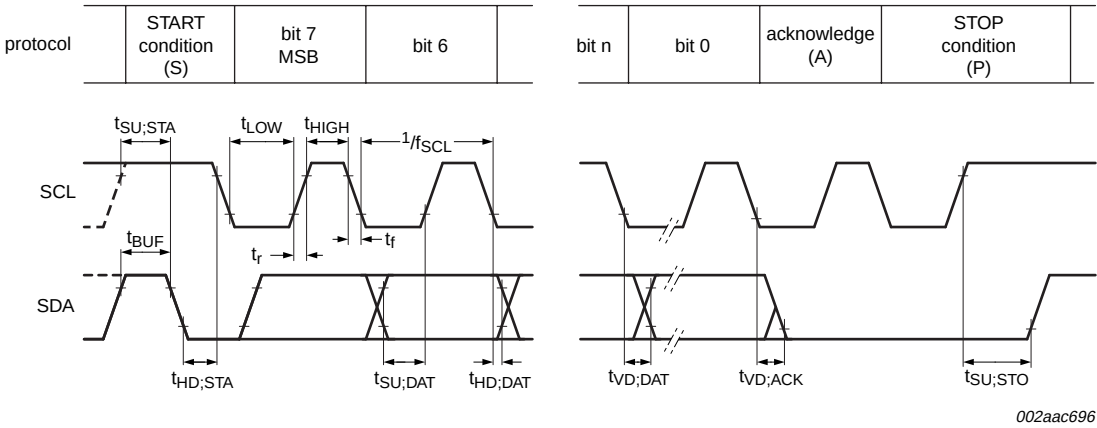
Fig 43. I 2 C-bus timing diagram
