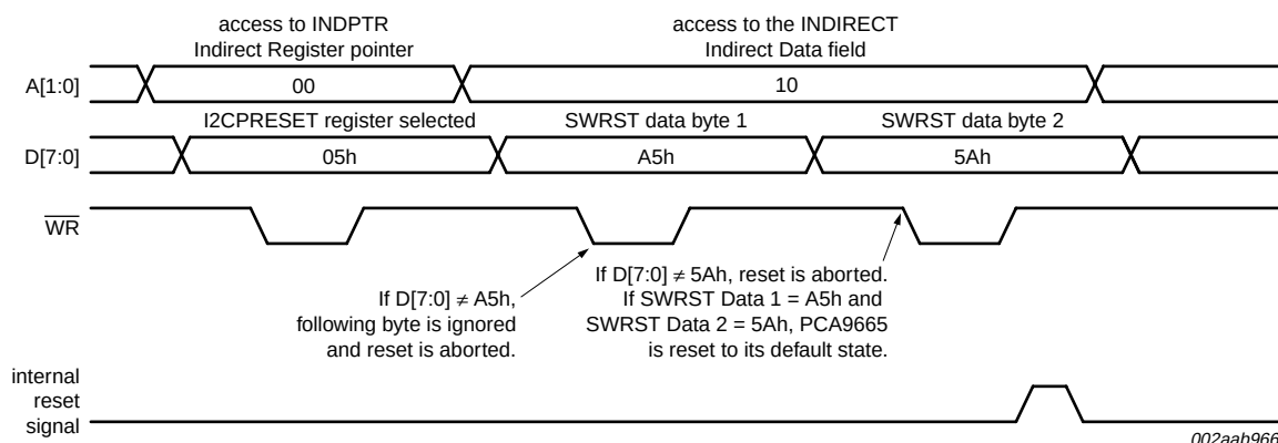
Fig 18. Parallel Software Reset sequence
