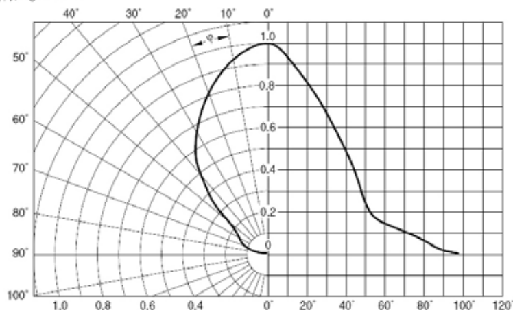
Radiation Characteristic
