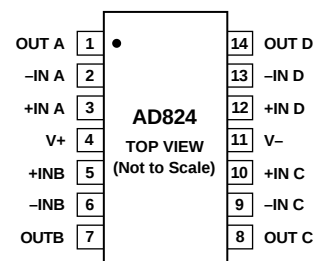
14-Lead Epoxy SO (R Suffix)
