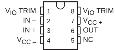
JG OR P PACKAGE (TOP VIEW)
