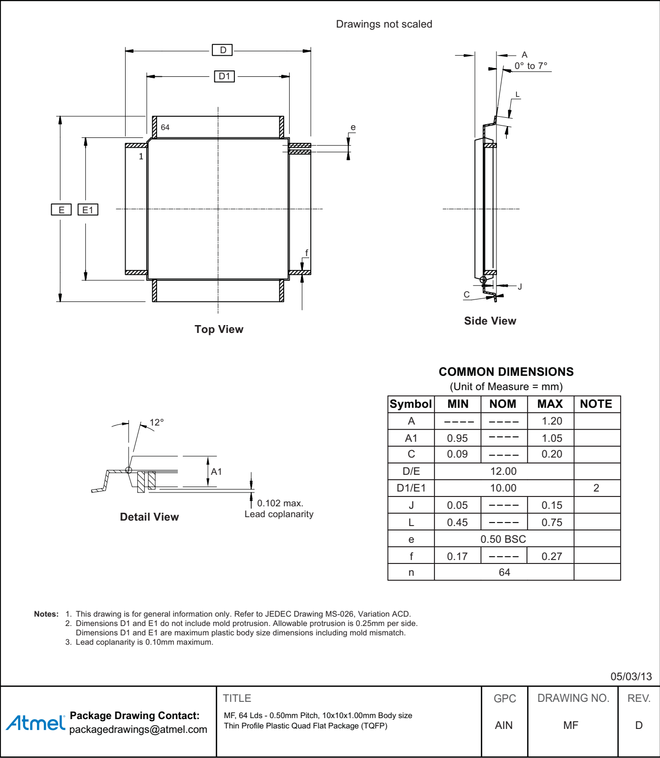
Figure 34-2. Package MF
