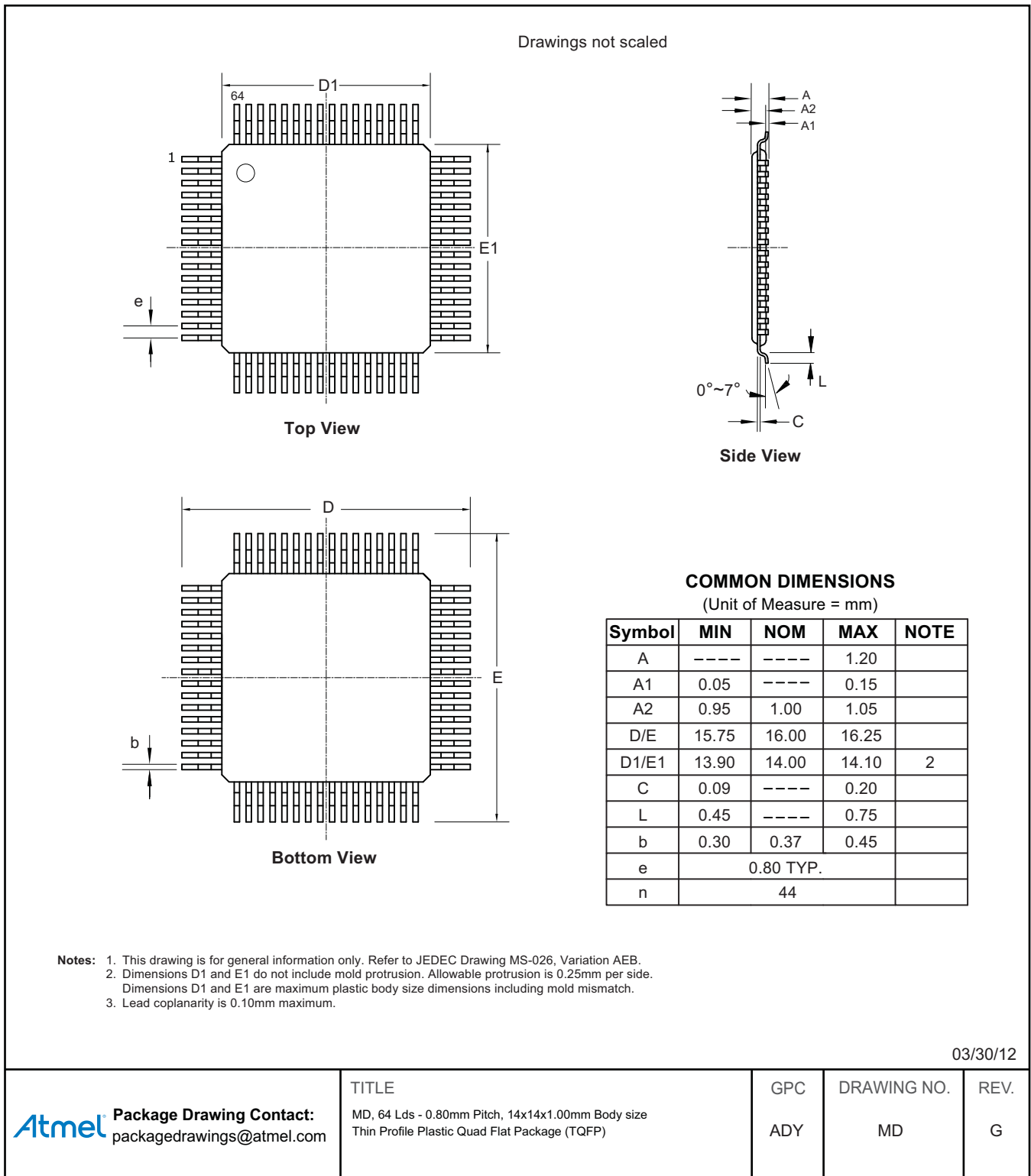
Figure 34-1. Package MD
