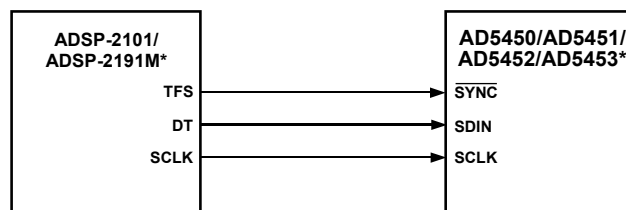
Figure 57. ADSP-2101/ADSP-2191M-to-AD5450/AD5451/AD5452/AD5453 Interface
