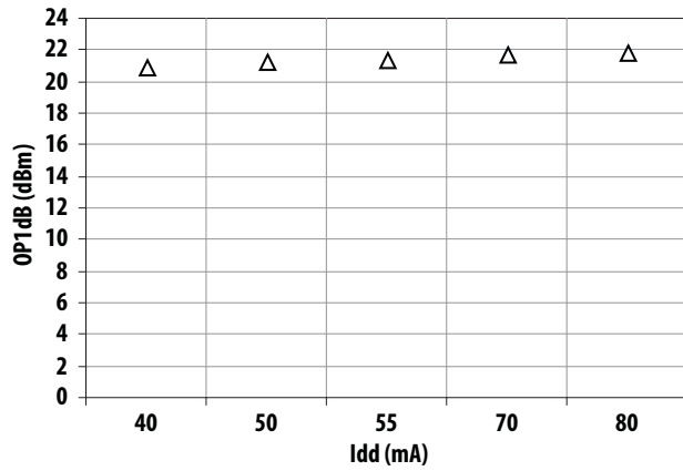
Figure 13. OP1dB vs Idd at 5V Tuned for Optimum OIP3 and Fmin at 1.9GHz
