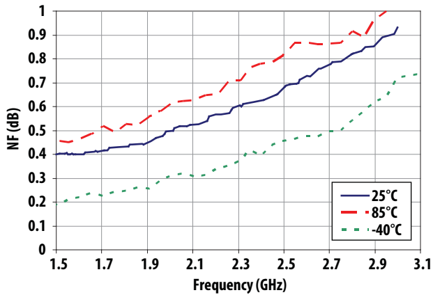
Figure 21. NF vs Frequency vs Temperature
