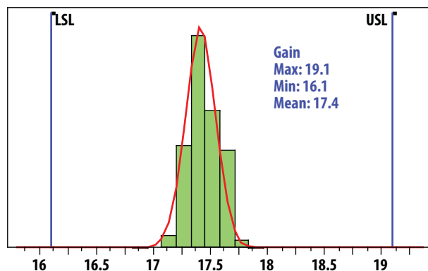
Figure 4. Gain @1.9GHz, 5V, 48mA Mean = 17.4
