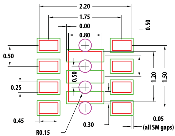
Land Pattern
