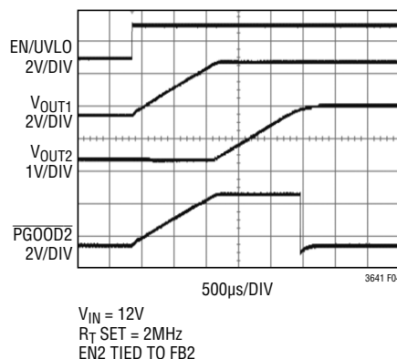
Figure 3. Soft-Start of LT3641
