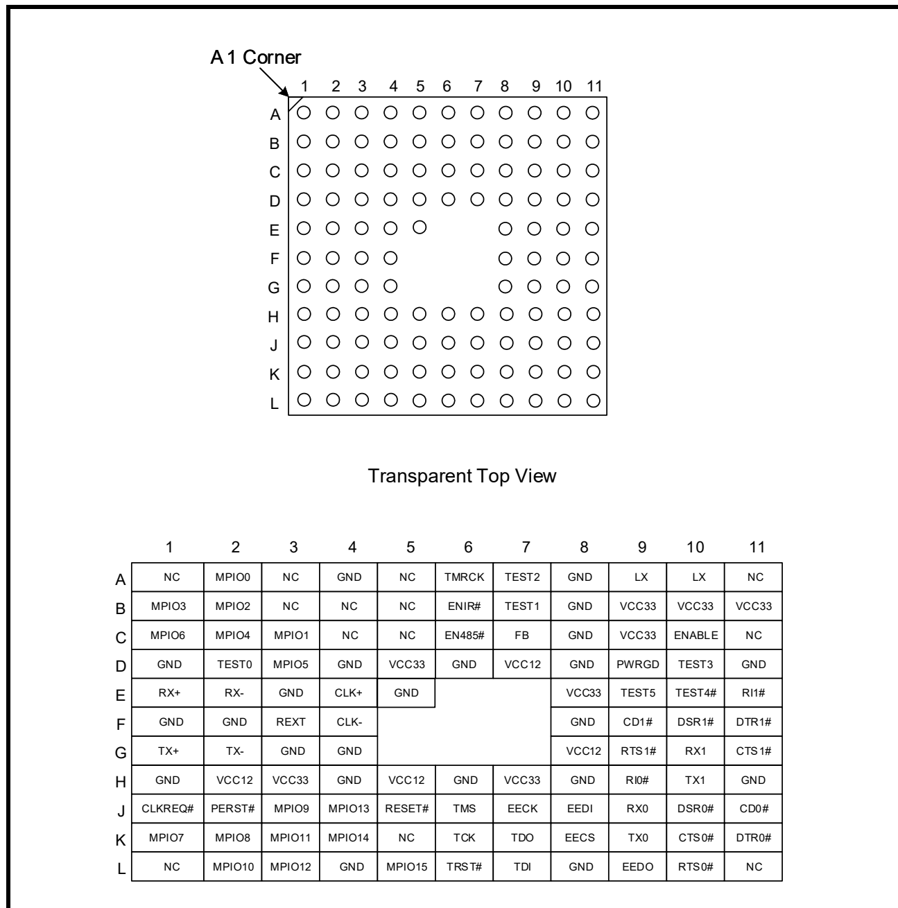
FIGURE 2. 113-FPBGA PINOUT
