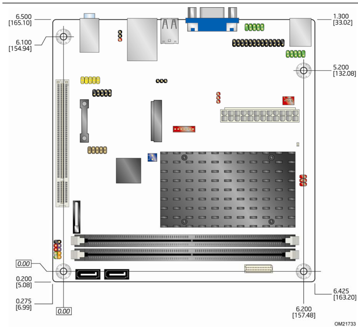
Figure 15. Board Dimensions
