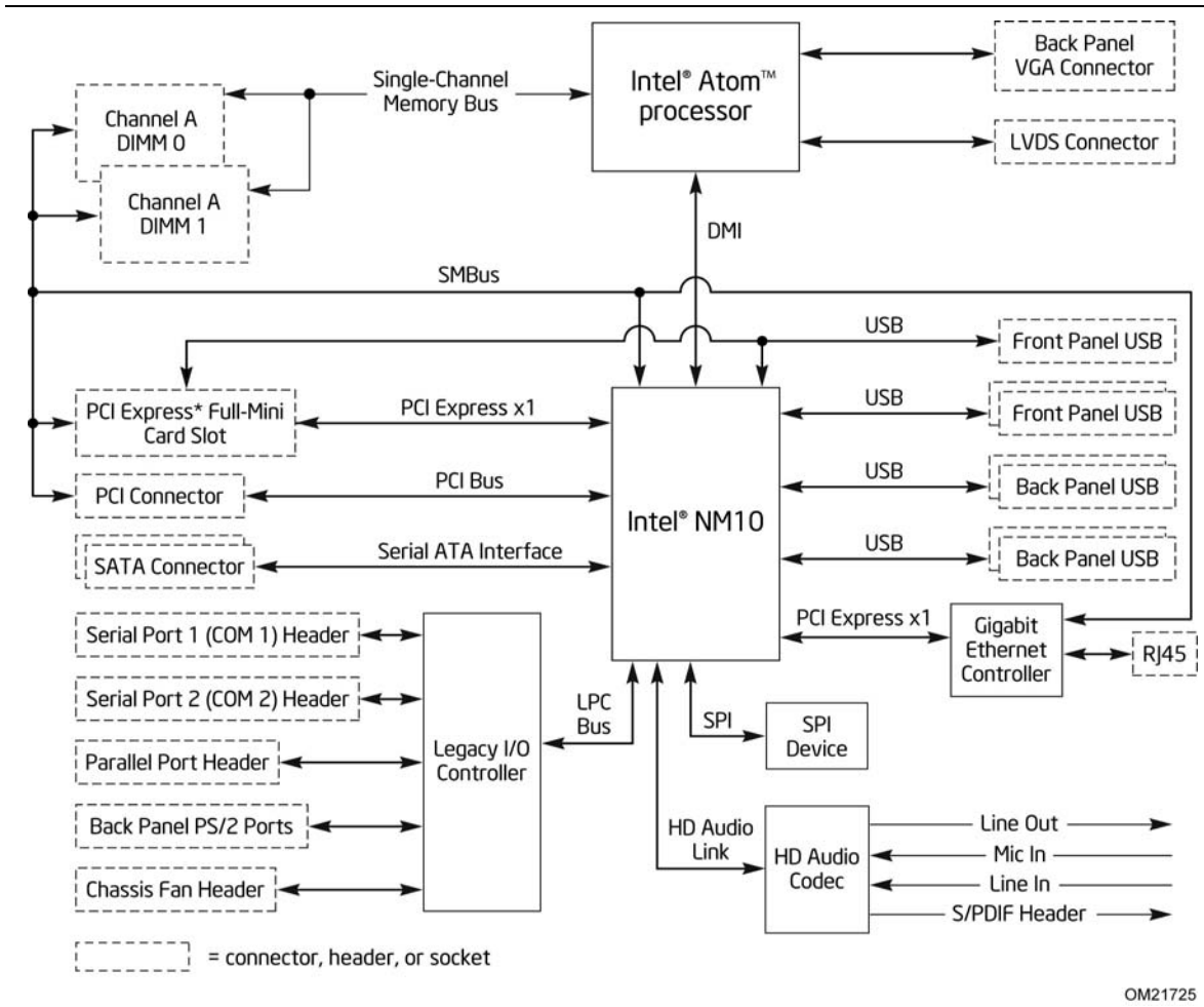
Figure 2. Block Diagram
