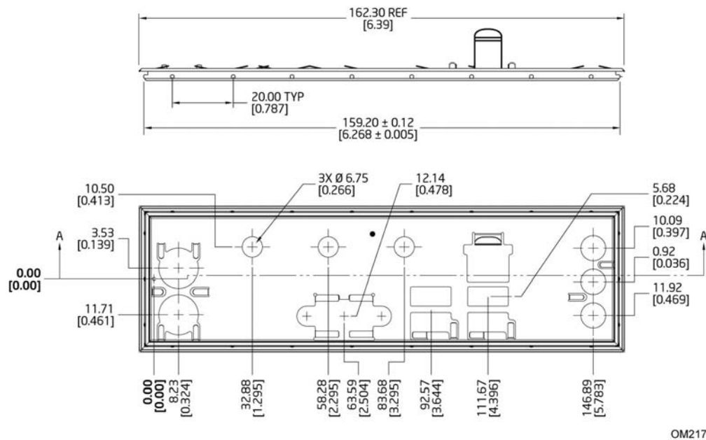
Figure 9. I/O Shield Reference Diagram
