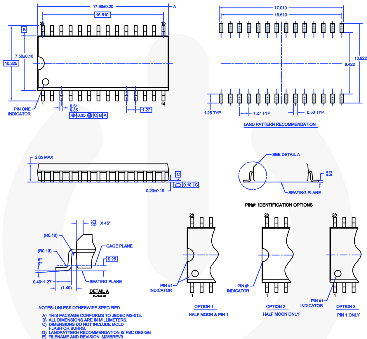
Figure 47.28-28-Lead Small Outline Integrated Circuit (28-Wide Body SOIC)
