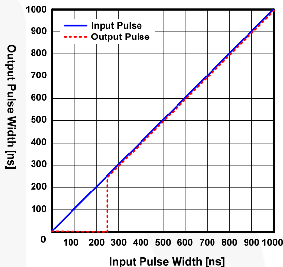
Figure 46. Input Filter Characteristic of Narrow ON
