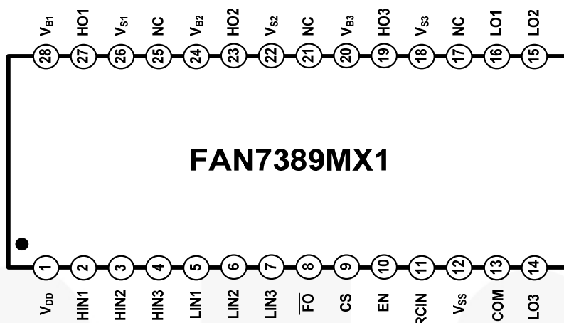
Figure 3. Pin Configuration
