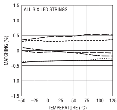
LED Current Matching
