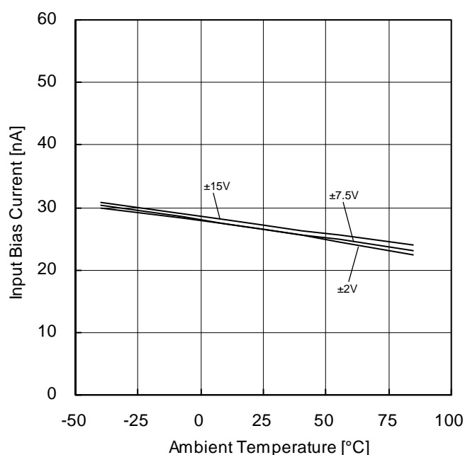
Figure 13. Input Bias Current vs Ambient Temperature ( V_{ICM}=0V , E_K=0V )
