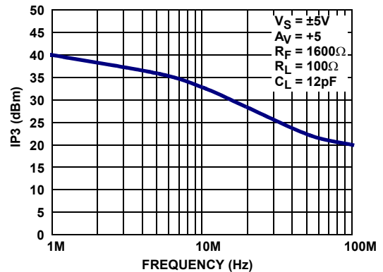
FIGURE 36. THIRD ORDER IMD INTERCEPT vs FREQUENCY
