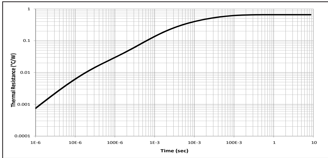
Fig 6. Transient Thermal Impedance, Junction - Case
