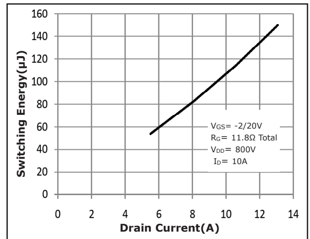
Fig 8. Inductive Switching Energy(Turn-off) vs ID
