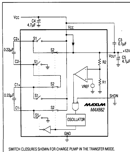
Figure 1. Block Diagram
