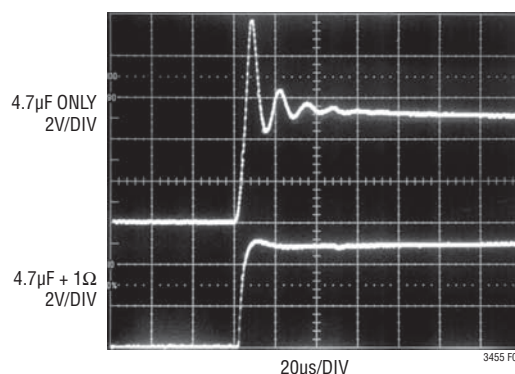
Figure 6. Waveforms Resulting from Hot-Plugging a 5V Input Supply
