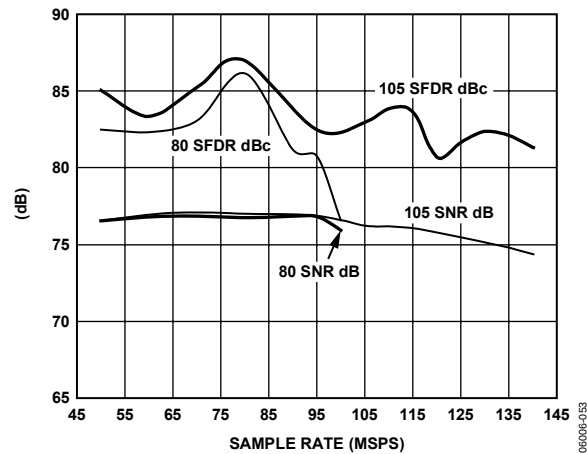
Figure 43. Single-Tone SNR/SFDR vs. Sample Rate, 170.3 MHz
