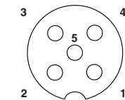
M12 slot, socket, 5-pos.
