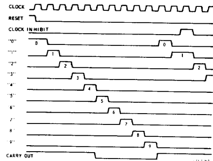
Fig. 2 - Timing diagram.
