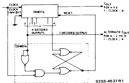
Fig. 12 – Divide by N counter (N ≤ 10) with N decoded outputs.
