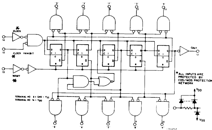
Fig. 1 - Logic diagram.
