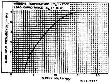
Fig. 7 — Typical clock input frequency vs. V_{DD} .
