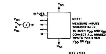
Fig. 10 – Input-leakage-current test circuit.
