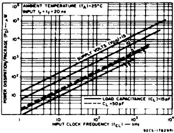
Fig. 8 — Typical dissipation characteristics.
