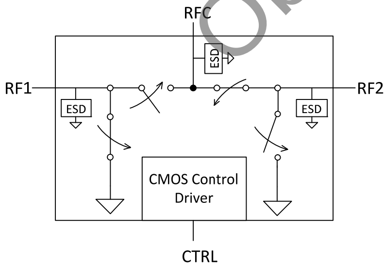
Figure 1. Functional Diagram
