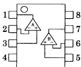
NJM13404D/13404M NJM13404E/13404V/13404R
