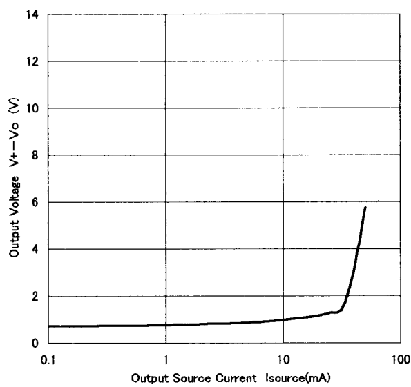
NJM13404 Output Voltage v.s Output Source Current
