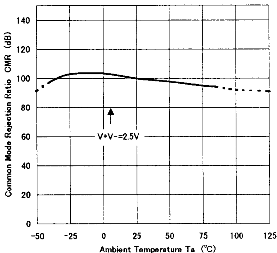
NJM13404 Common Mode Rejection Ratio vs. Temperature
