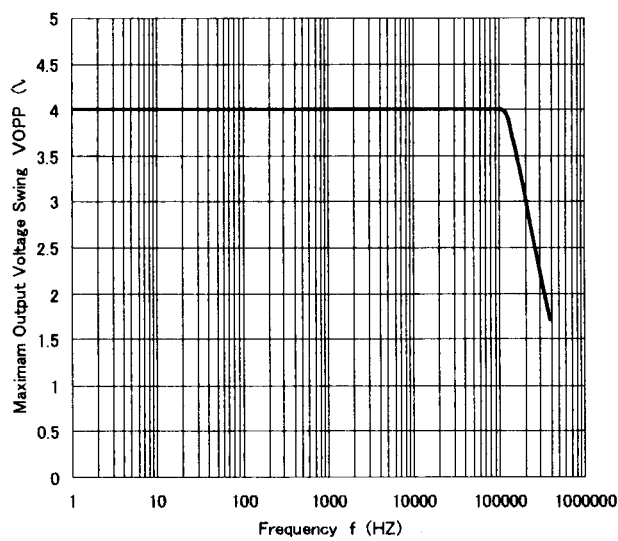
NJM13404 Maximum Output Voltage Swing v.s Frequency
