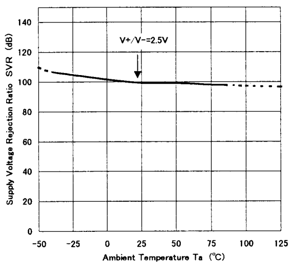
NJM13404 Supply Voltage Rejection Ratio vs. Temperature
