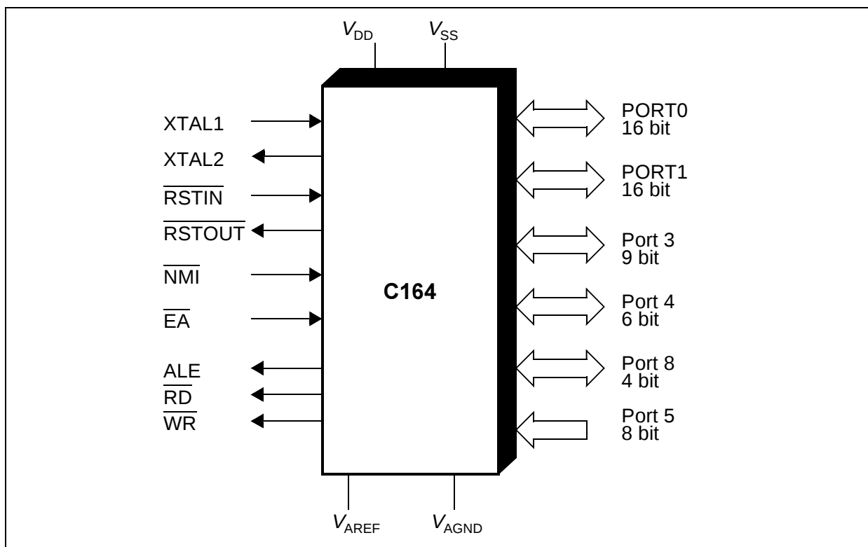
Figure 1 Logic Symbol
