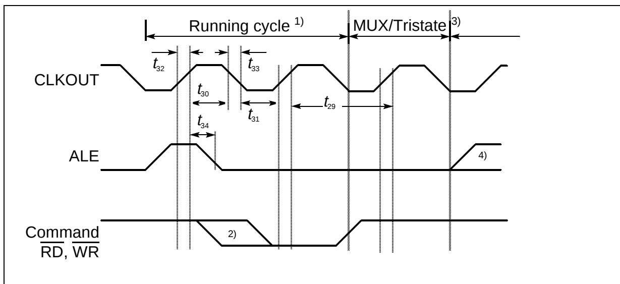
Figure 23 CLKOUT Timing
