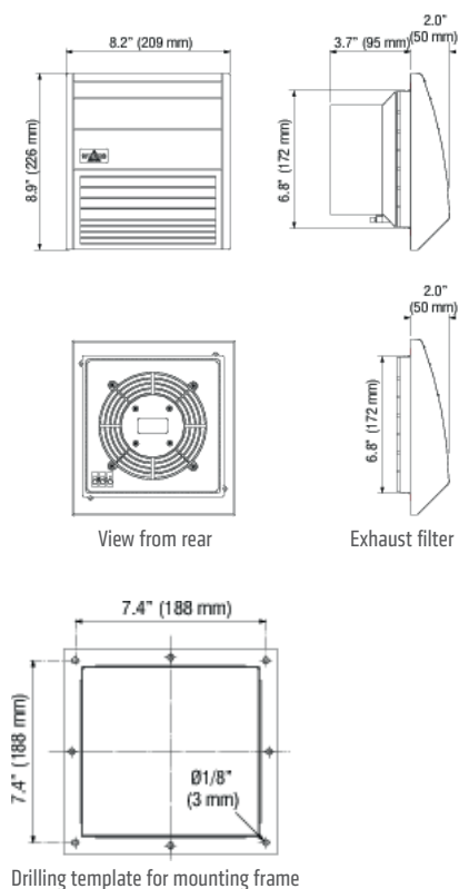
Drilling template for mounting frame
