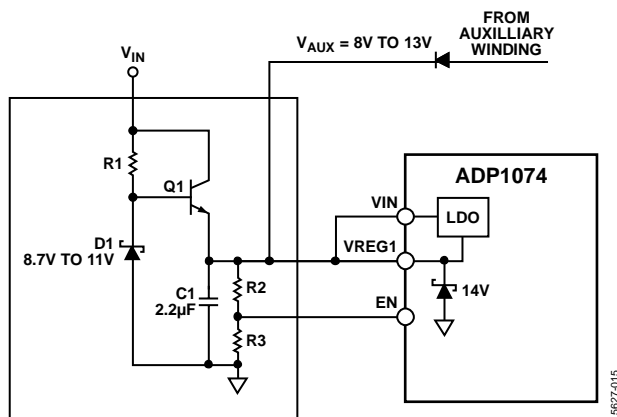
Figure 15. Fast Start-Up Circuit
