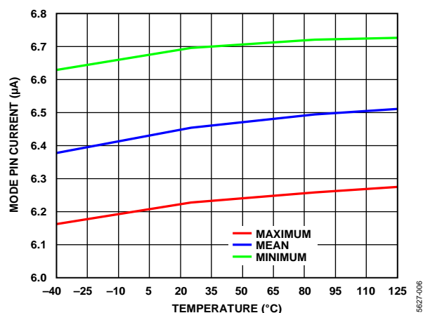
Figure 6. MODE Pin Current vs. Temperature
