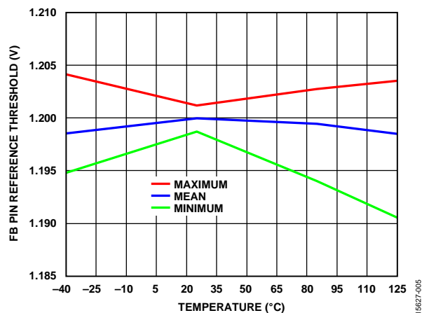
Figure 5. FB Pin Reference Threshold vs. Temperature
