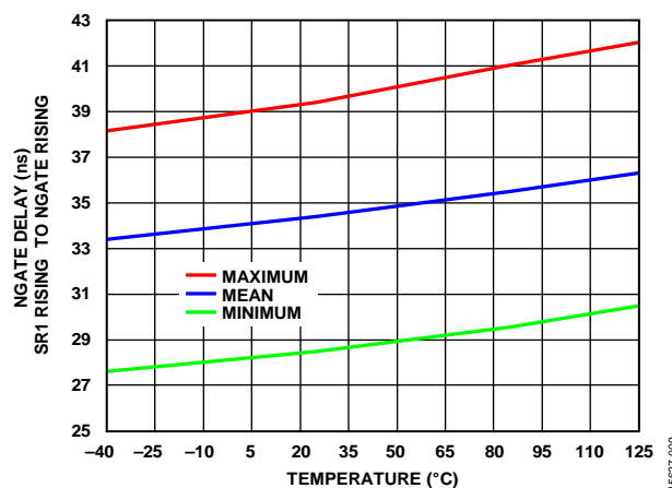
Figure 9. NGATE Delay (SR1 Rising to NGATE Rising) vs. Temperature
