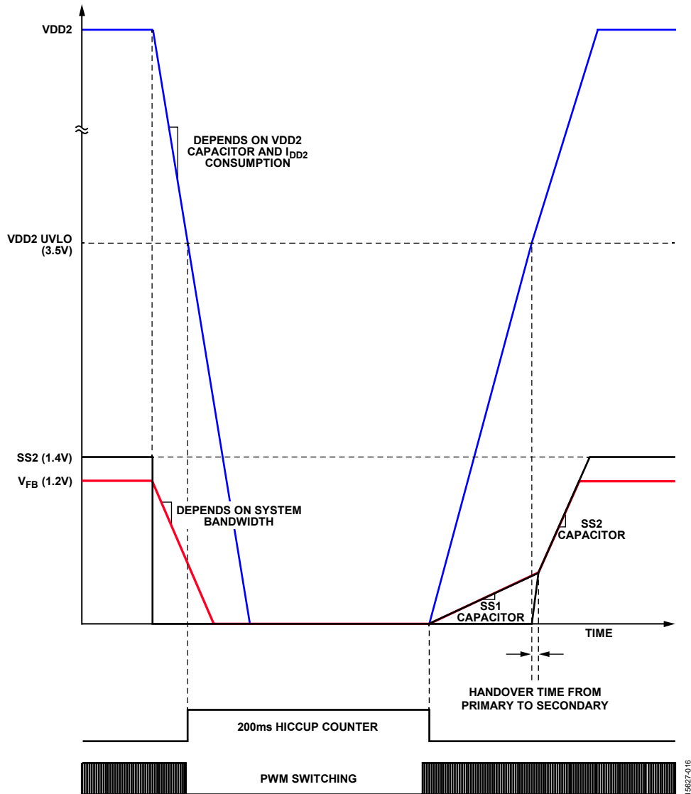
Figure 16. Remote Software Reset with 200 ms Hiccup
