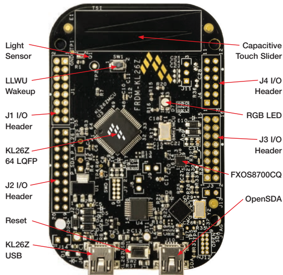
Figure 1: FRDM-KL26Z Callouts
