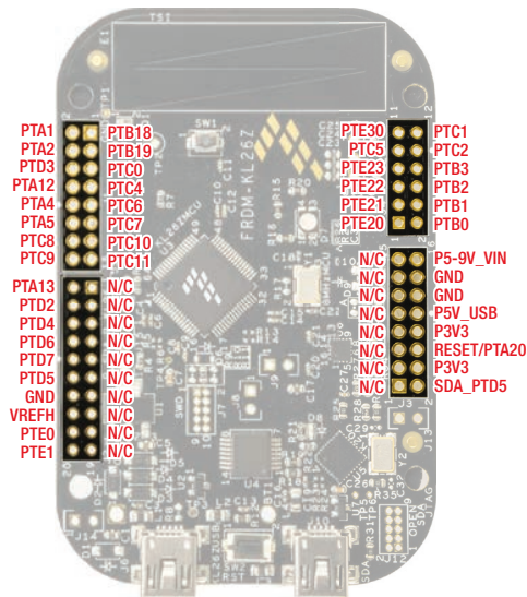
Figure 2: FRDM-KL26Z Pin-Out
