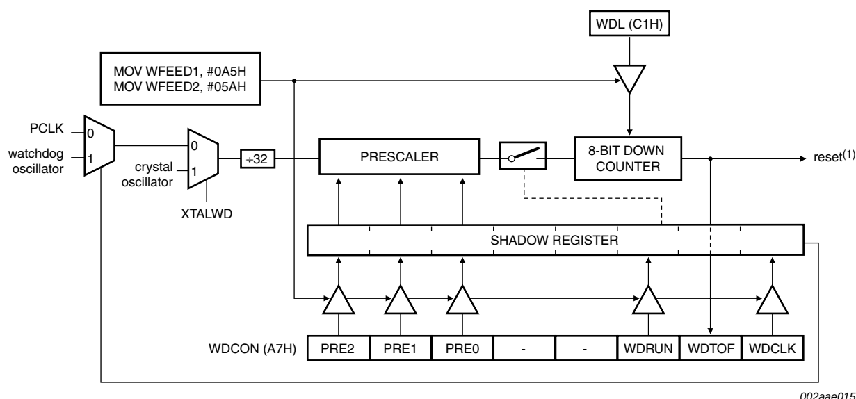
Fig 20. Watchdog timer in Watchdog mode (WDTE = 1)
