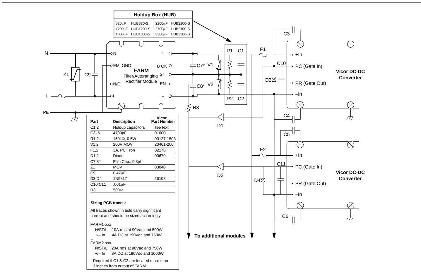
Figure 9—Converter connections
