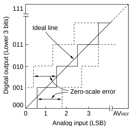
Figure 10-14. Zero-Scale Error
