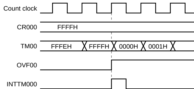
Figure 6-36. Operation Timing of OVF00 Flag
