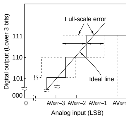
Figure 10-15. Full-Scale Error
