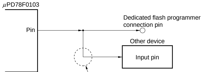
Figure 21-15. Malfunction of Other Device
