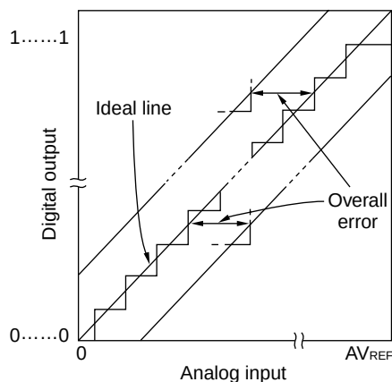
Figure 10-12. Overall Error
