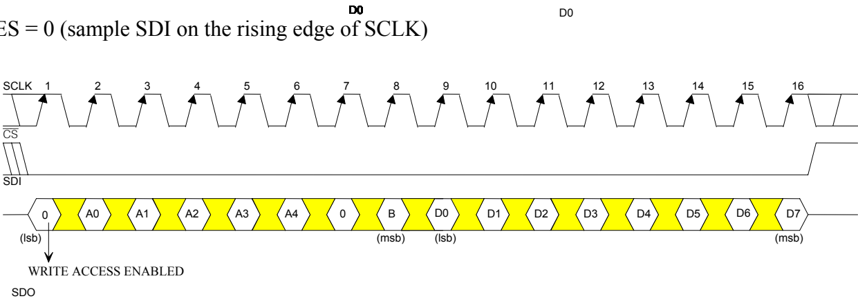
Figure 3-6. Serial Port Operation for Write Access (R = 0) Modes 3 and 4
