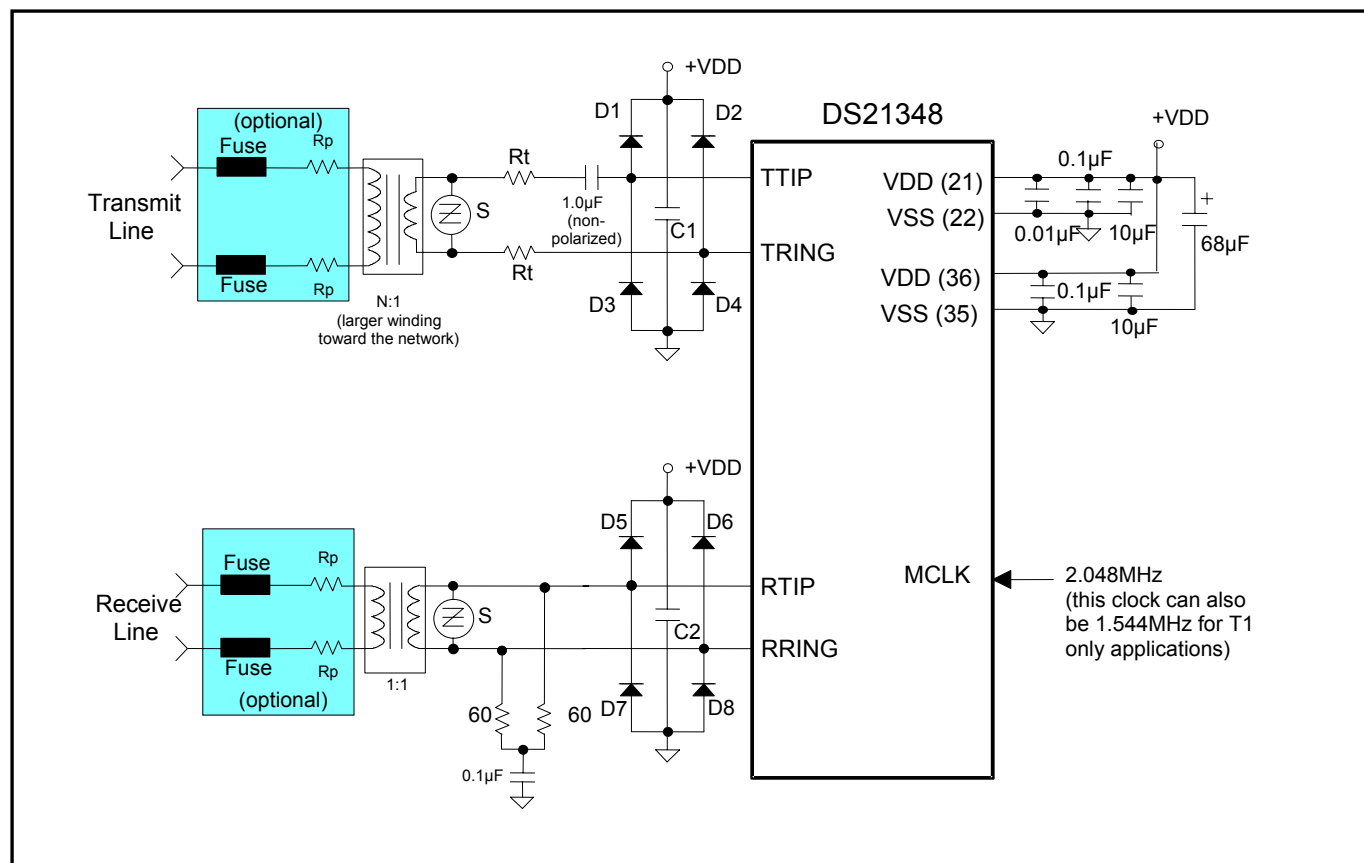
Figure 7-2. Protected Interface Using Internal Receive Termination
