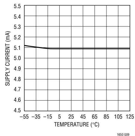
AVDD Supply Current vs Temperature
