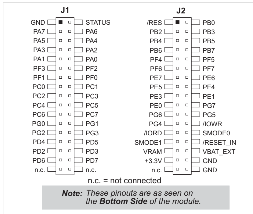
Figure 5. RCM3000 Pinouts
