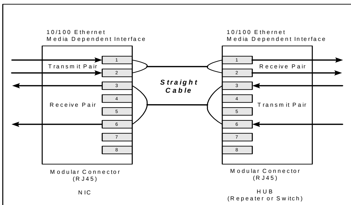
Figure 1: Typical Straight Cable Connection
