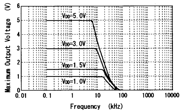
Maximum Output Swing Voltage vs. Frequency
