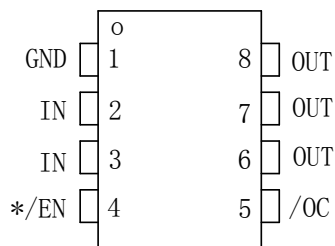
PI5PD2061/65 SOIC-8 and EP-MSOP-8 (Top View)
