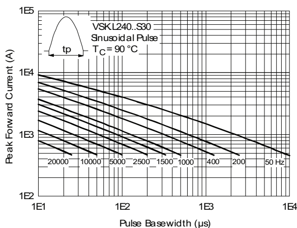
Fig. 25 - Frequency Characteristics
