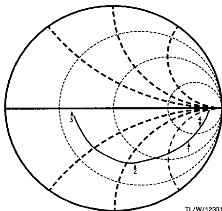
RF Input Impedance
