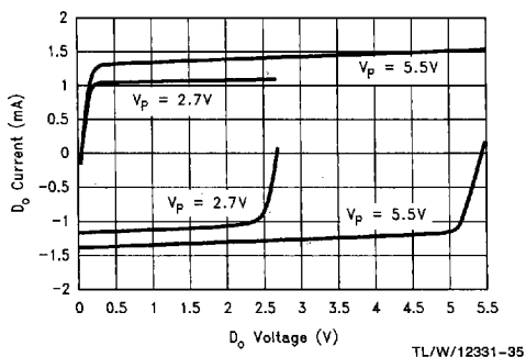
Sink vs Source Mismatch (See Note 2 under Charge Pump Current Specification Definitions)
