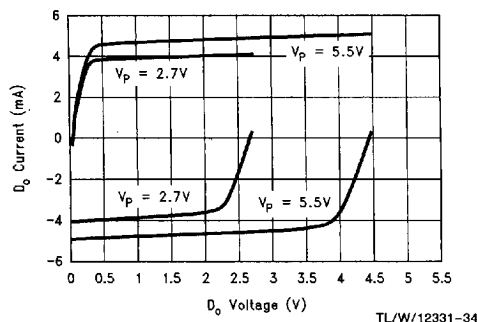
Charge Pump Current Variation (See Note 1 under Charge Pump Current Specification Definitions)
