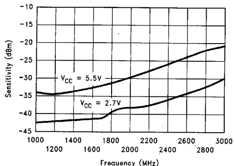
LMX2330A RF Sensitivity vs Frequency
