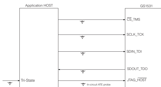
Figure 4-11: System JTAG
