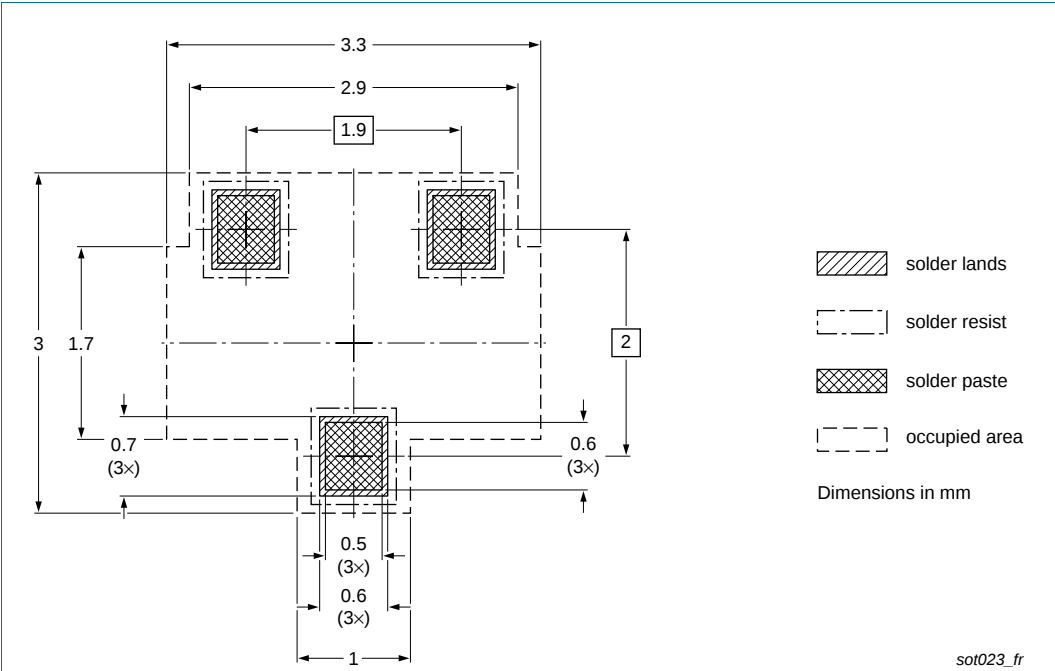
Fig 18. Reflow soldering footprint PDTA143XT (SOT23)
