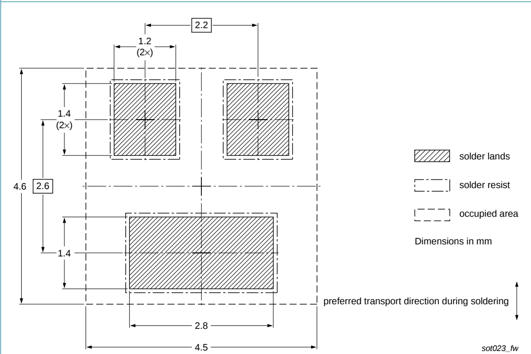
Fig 19. Wave soldering footprint PDTA143XT (SOT23)
