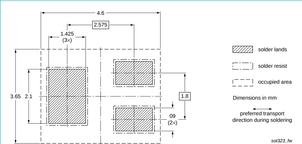
Fig 21. Wave soldering footprint PDTA143XU (SOT323/SC-70)
