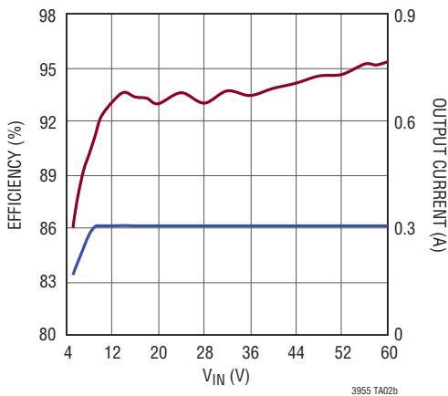
Boost Efficiency, Output Current vs V_{IN}
