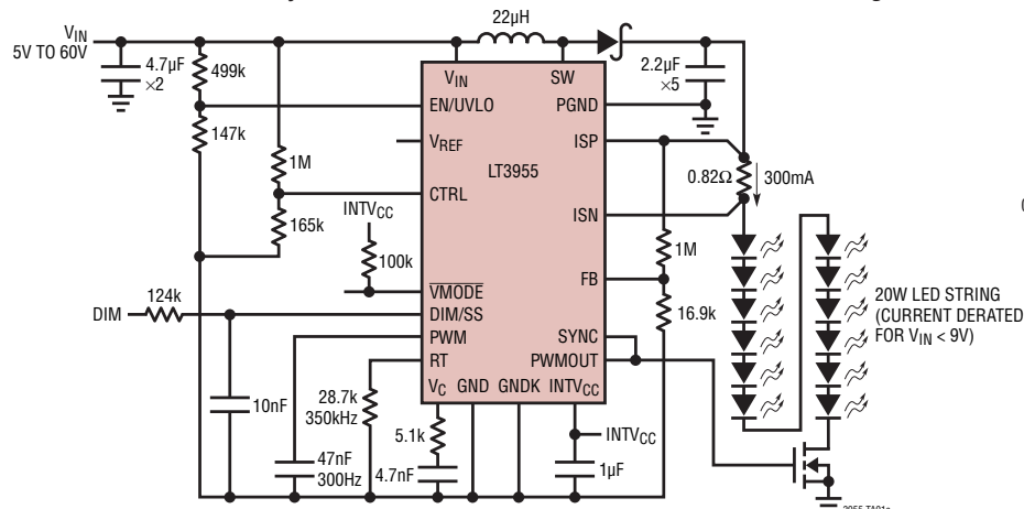
94% Efficiency 20W Boost LED Driver with Internal PWM Dimming
