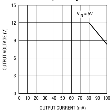
Output Voltage
