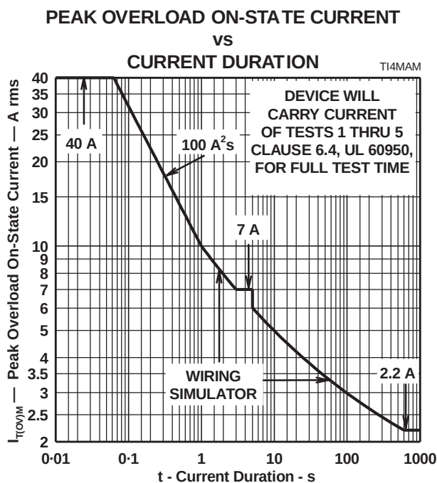
Figure 10. Peak Overload On-State Current against Duration
