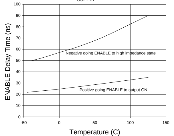
Fig. 32 ENABLE Propagation vs. Temperature V SUPPLY = 15V
