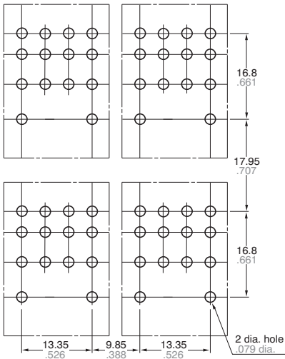
Side-by-side installation
