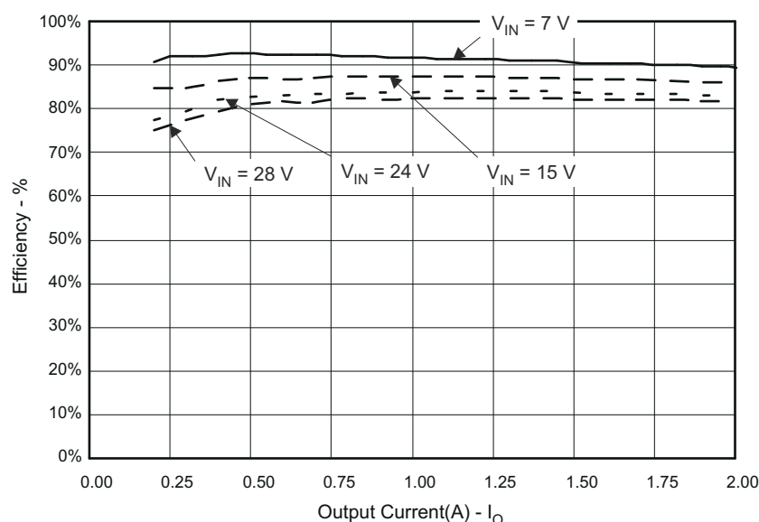
Figure 2-1. TPS54231EVM-372 Efficiency
