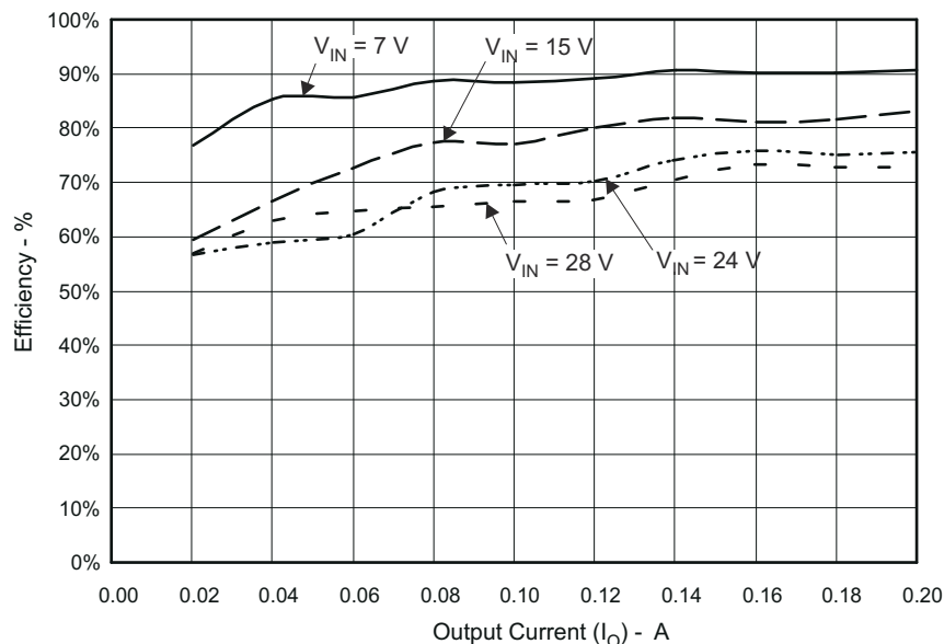
Figure 2-2. TPS54231EVM-372 Low Current Efficiency
